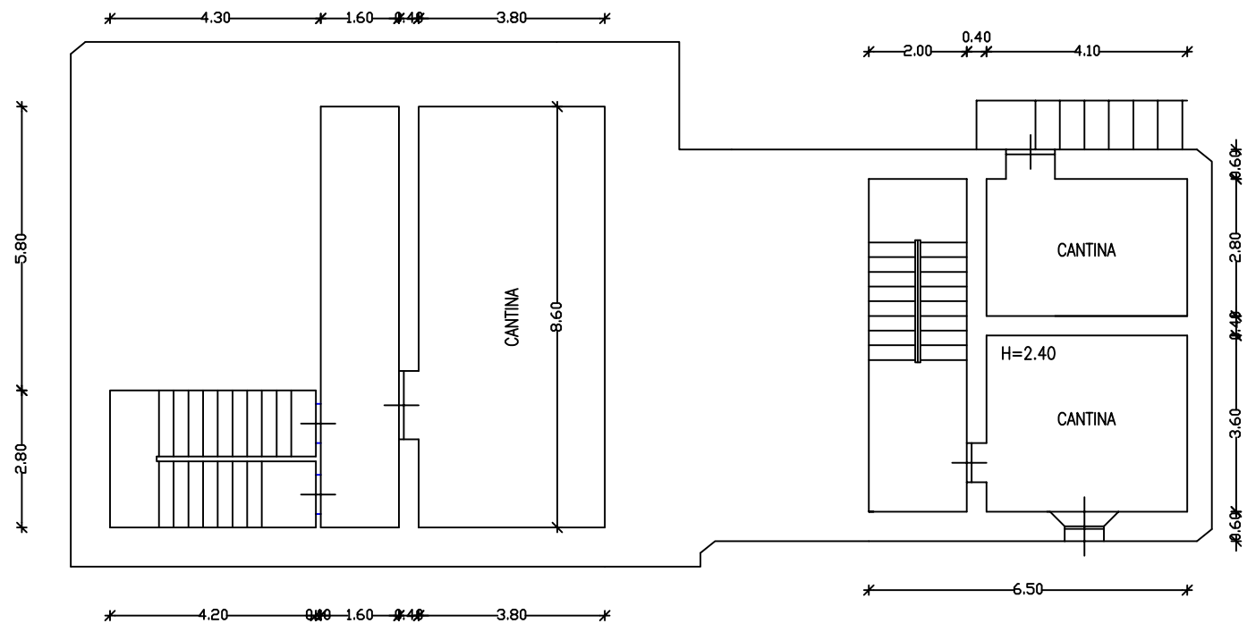
PIANO INTERRATO
